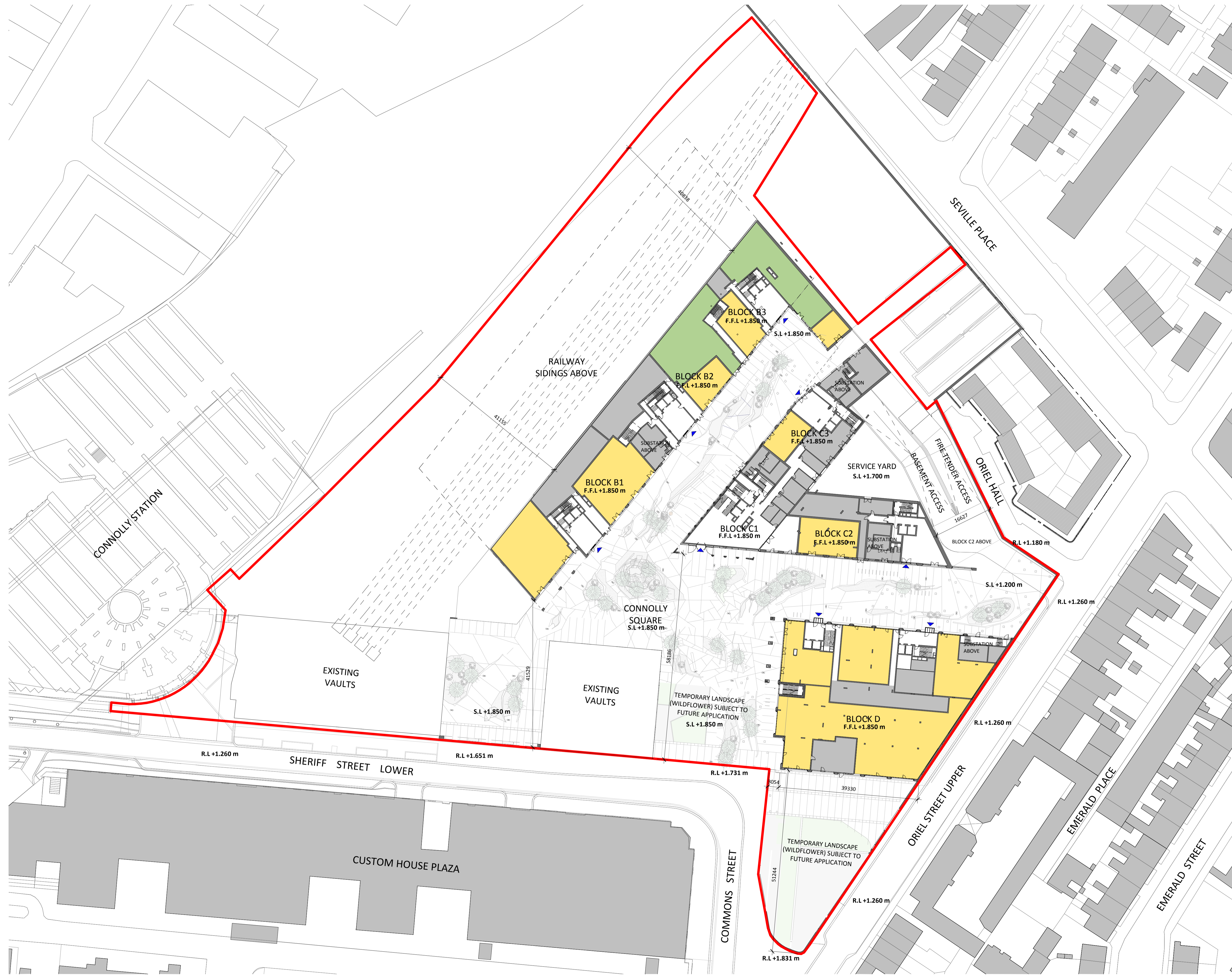
1 SITE LAYOUT PLAN - LEVEL 00 1 : 500
